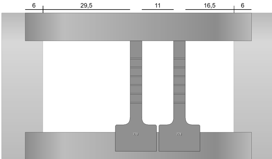
View fixed-point connection, all dimensions in mm
